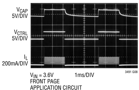
Transient Response
