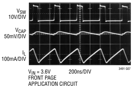
Switching Waveform
